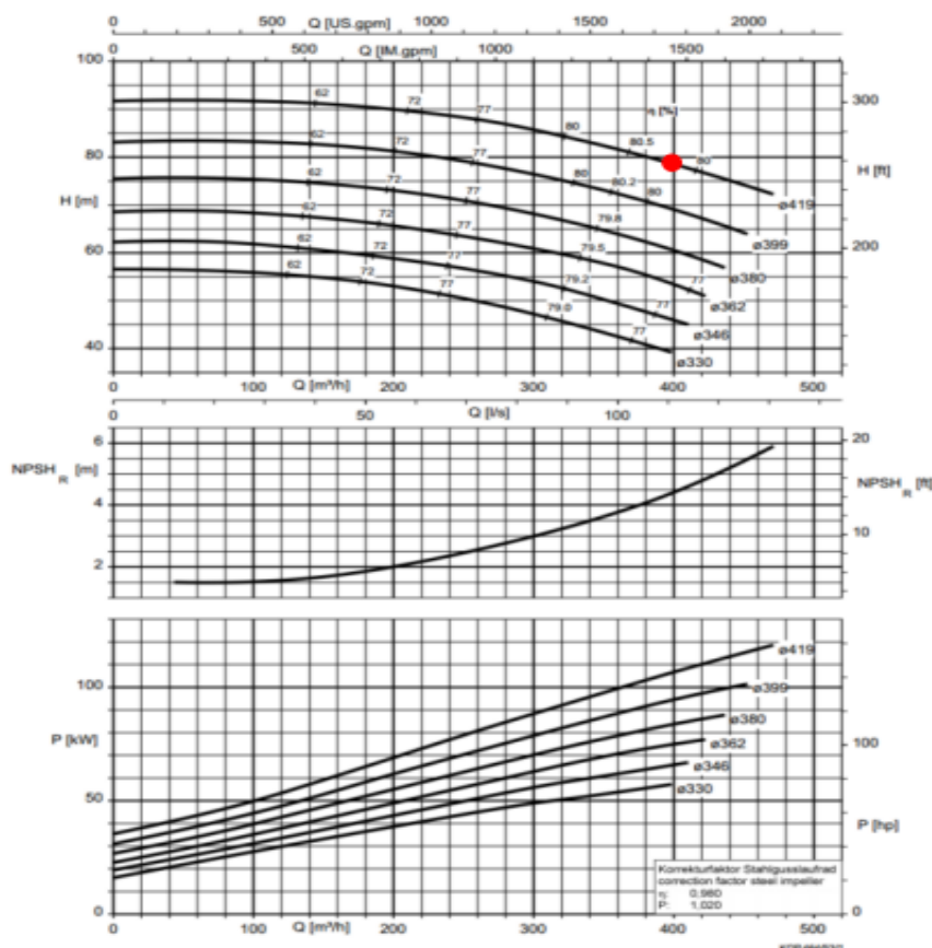
MegaCPK 150-125-400, n = 1750 r.p.m. Meganorm
